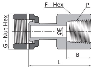
FR Welded Gland to Female NPT
